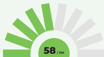
SCORE GLOBAL
